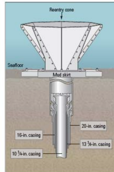
▲ The reentry cone. A large 3.7-m [12-ft] diameter, funnel-shaped installation on the seafloor serves as a conduit for relocating a previously drilled hole and for landing and supporting the surface casing string. The reentry cone is released through the moon pool (top). (Photograph courtesy of Texas A&M University.)
