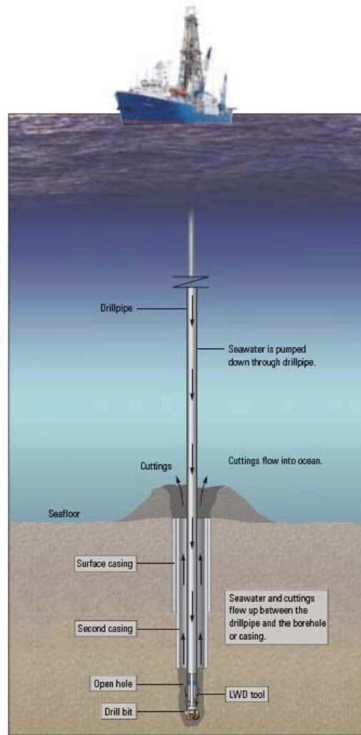
^ Riserless drilling. Seawater is pumped down through the drillpipe to clean and cool the bit. The drilling fluid and the cuttings flow up between the drillpipe and the borehole or casing, where they spill onto the seafloor and do not return to the surface.
