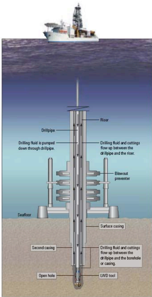
^ Riser drilling. The riser is a pipe that extends from the drilling platform down to the seafloor. Drilling mud and cuttings from the borehole are returned to the surface through the riser. The top of the riser is attached to the drillship, while its bottom is secured at the seafloor. A blowout preventer (BOP) placed at the seafloor between the wellhead and the riser provides protection against overpressured formations and sudden release of gas. The riser pipe diameter of up to 21 in. (53.3 cm) is large enough to allow the drillpipe, logging tools and multiple casing strings to pass through.
